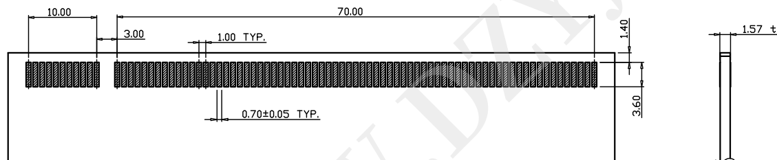
RECOMMENDED PCB LAYOUT TOLERANCE: ±0.05
