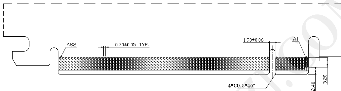
RECOMMENDED EDGE CARD PATTERN(SECONDARY SIDE)
