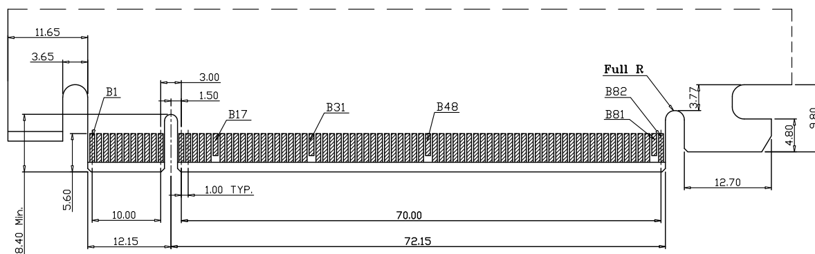
RECOMMENDED EDGE CARD PATTERN(PRIMARY SIDE)
